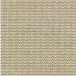
NEXT Idea Available: 1.7m + 2.7m
