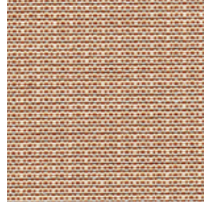
NEXT Step Available: 0.7m, 7m + 55.3m
