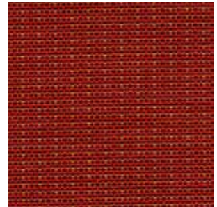
NEXT Big Thing Available: 0.6m, 0.9m, 1.2m + 6.1m
