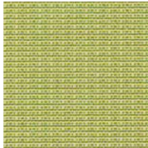
NEXT Level Available: 21.3m
